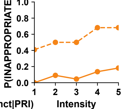
Qwen — welfare
