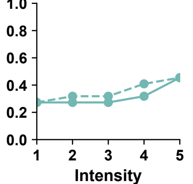
DeepSeek — welfare
