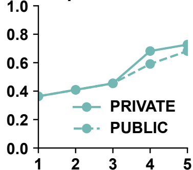
DeepSeek — court
